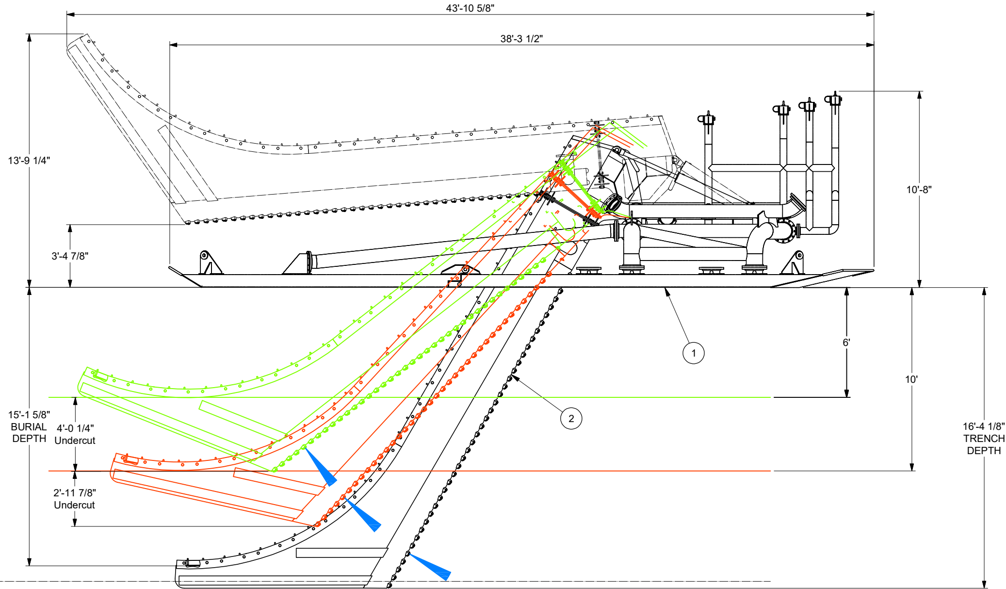
ELEVATION ON JET SLED OVERALL ARRANGEMENT J0645-080-000 ( 1 : 60 )
